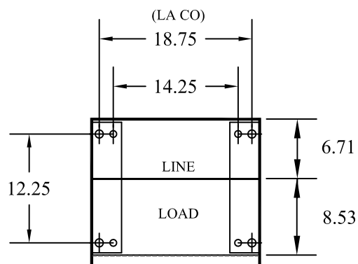
FRONT MOUNTING PLAN
