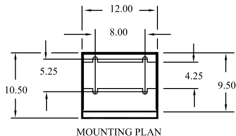
MOUNTING PLAN CAL TRANS TYPE III-AF
