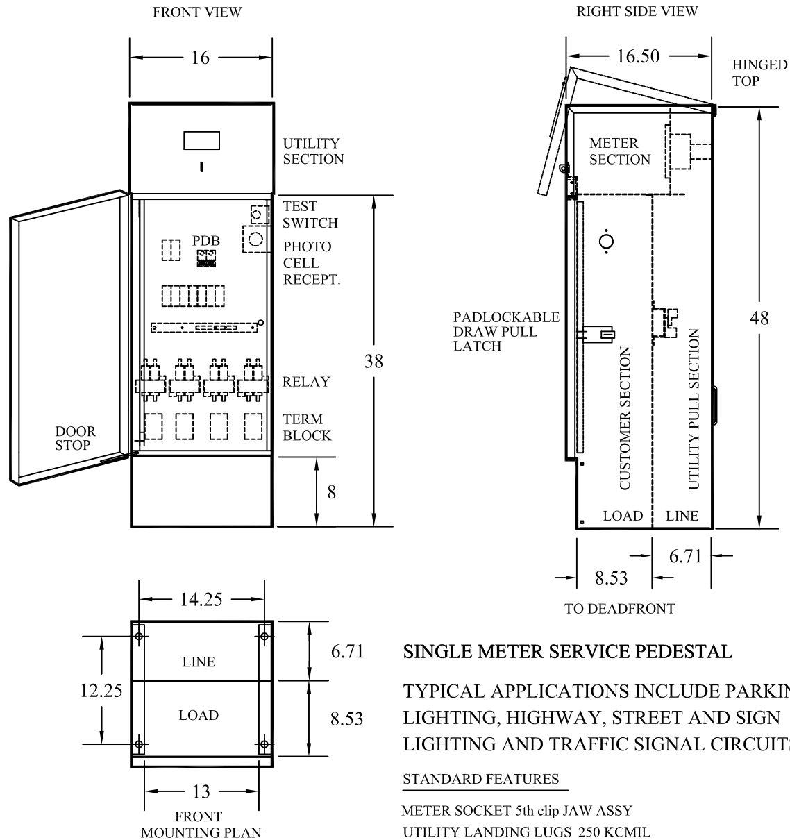
STANDARD PEDESTAL OF MISSOURI DEPARTMENT OF TRANSPORTATION
