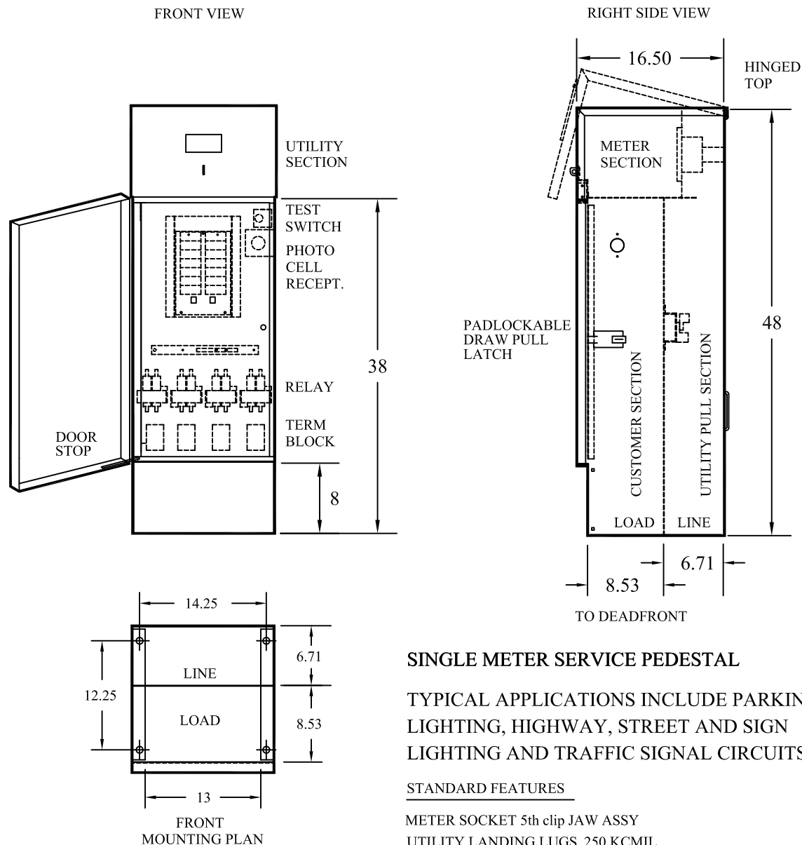
STANDARD PEDESTAL OF MISSOURI DEPARTMENT OF TRANSPORTATION
