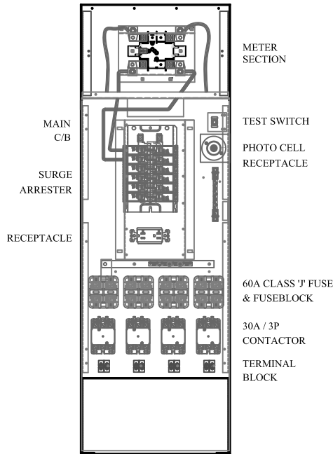
FRONT VIEW SHOWN LESS DOOR & COVERS
