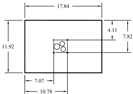
BOTTOM PLAN
