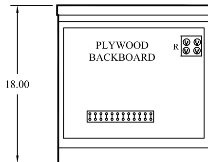
FRONT VIEW (LESS HINGED DOOR)
